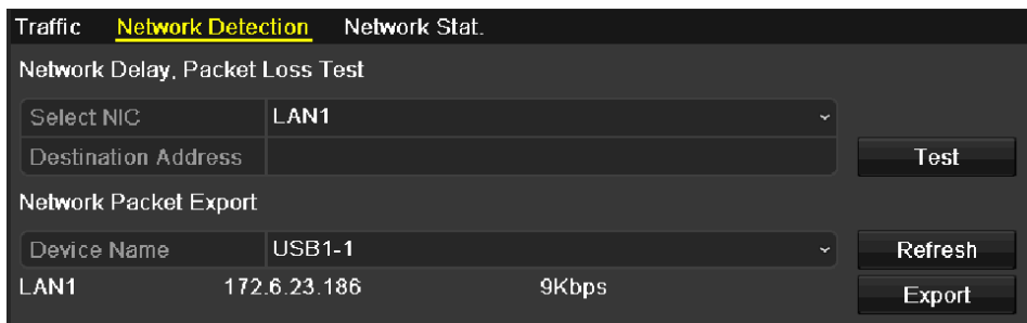
Figure 9.31 Export Network Packet
