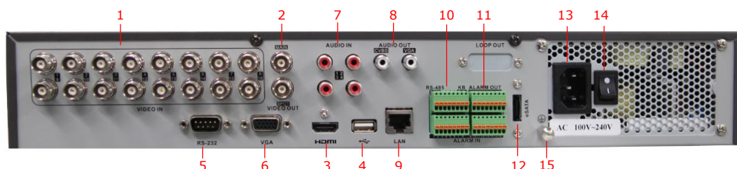
Figure 1.10 Rear Panel of DS-7316HFI-SH and DS-7316HWI-SH
