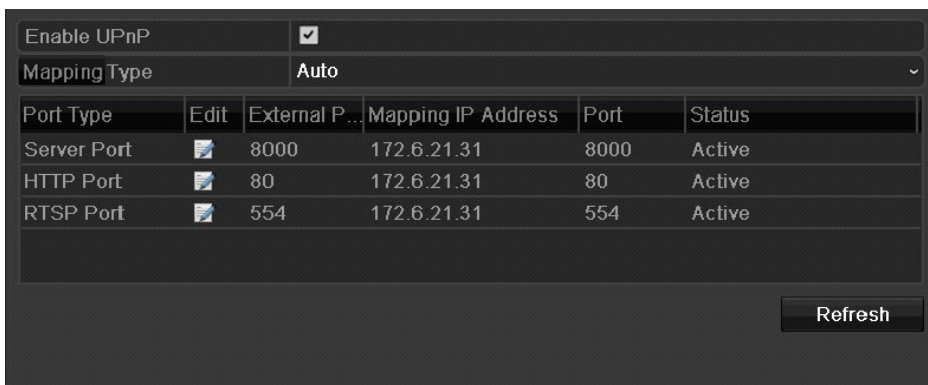
Figure 9.18 UPnP Settings Finished
