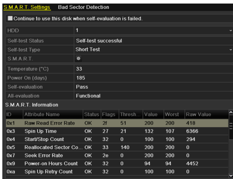
Figure 10.20 S.M.A.R.T. Settings Interface
