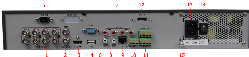
Figure 1.9 Rear Panel of DS-7308HFI-SH and DS-7308HWI-SH
