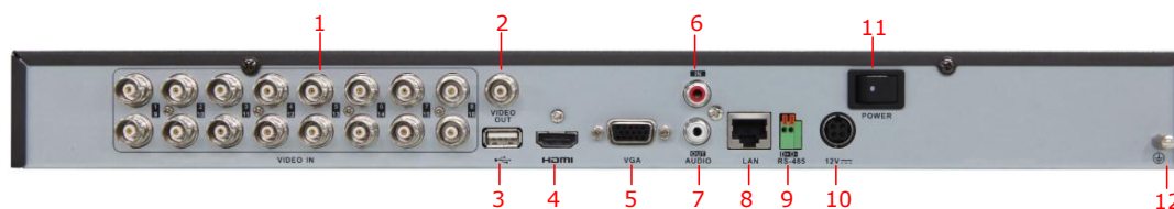
Figure 1.7 Rear Panel of DS-7216HFI-SH and DS-7216HWI-SH
