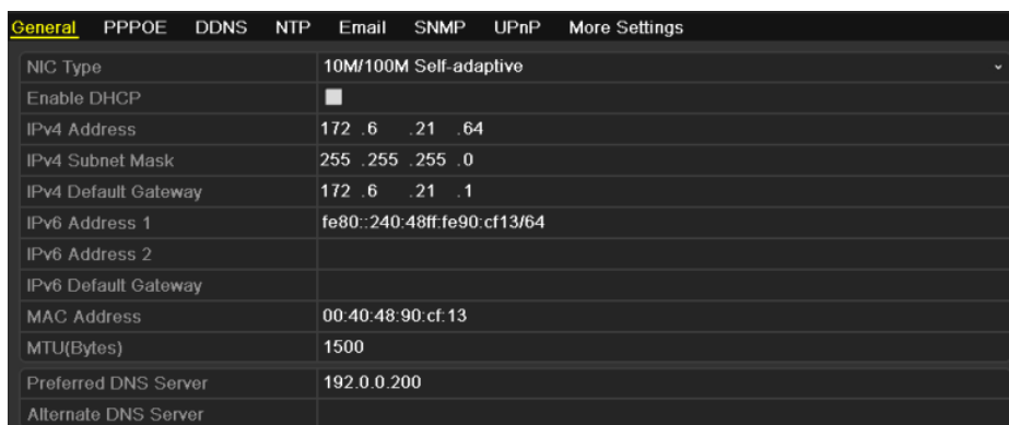
Figure 9.24 Network Settings Interface
