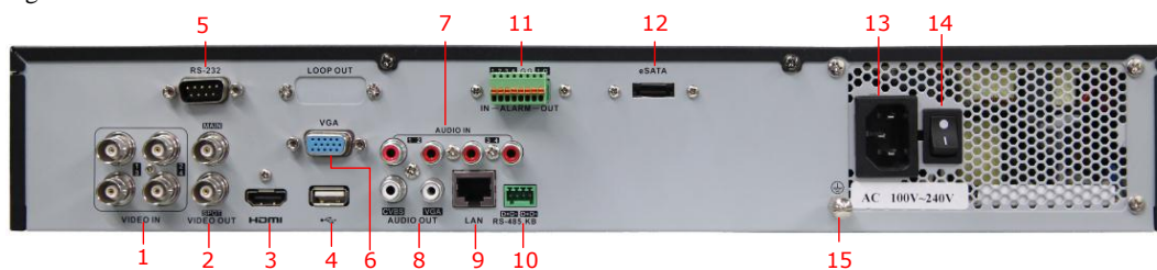
Figure 1.8 Rear Panel of DS-7304HFI-SH and DS-7304HWI-SH
